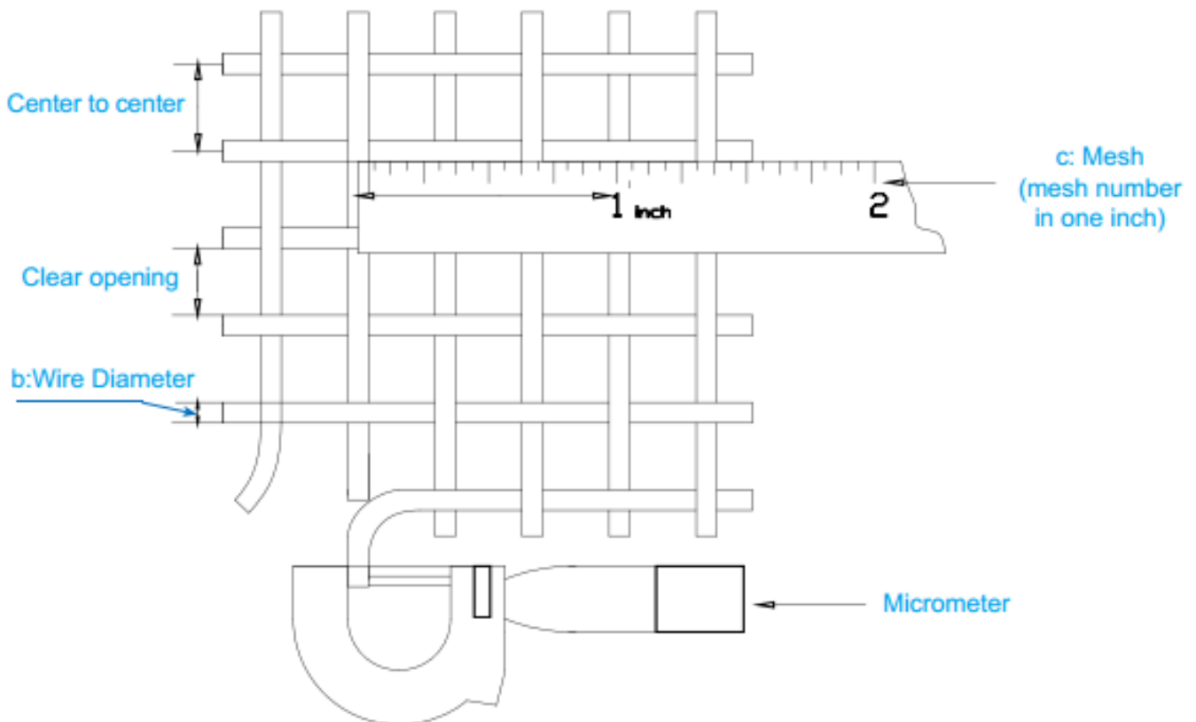
Size Marking of Stainless Steel Wire Mesh
